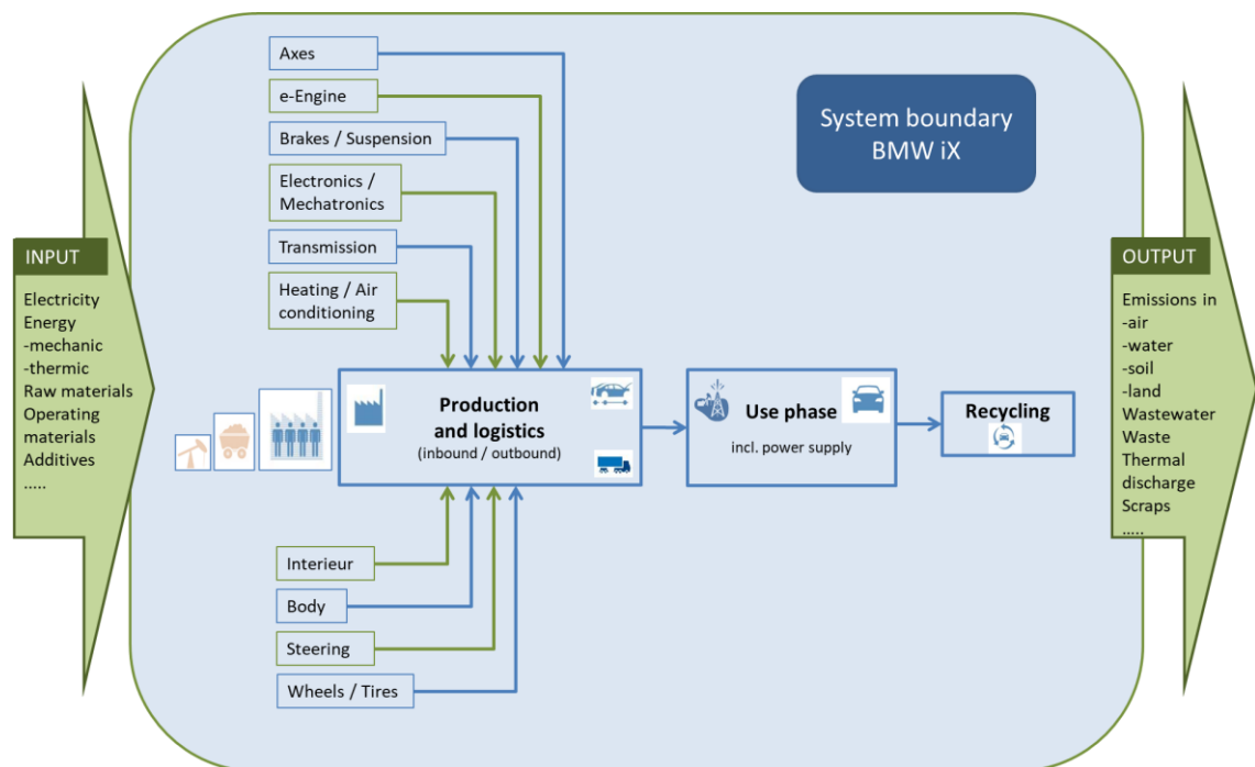
Fig. 1: Flowchart input / output data of the BMW iX
